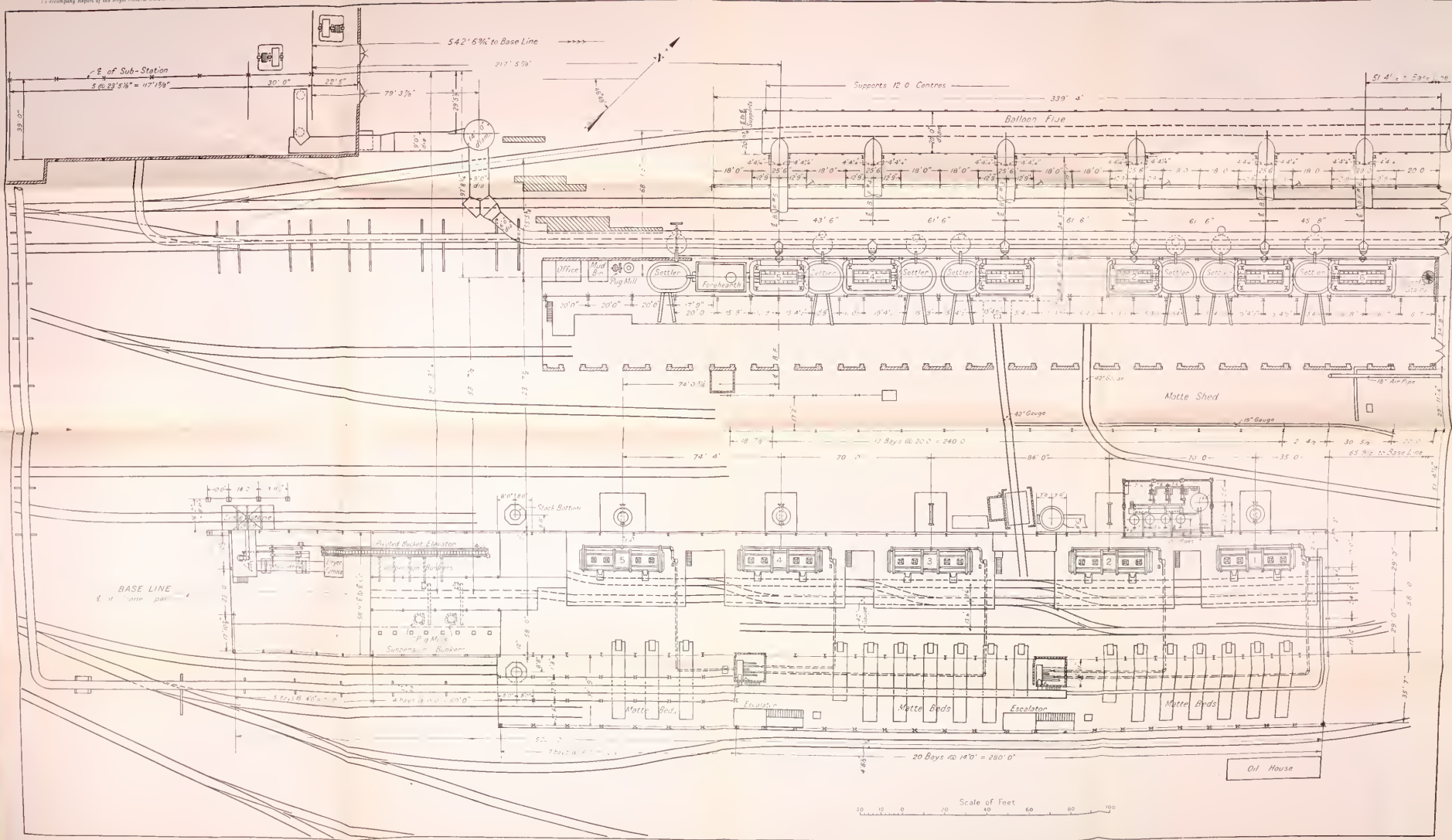
Plan and Layout of Ball Room and Converter Department, 1917, Canadian Copper Company, Copper Cliff, Ontario
